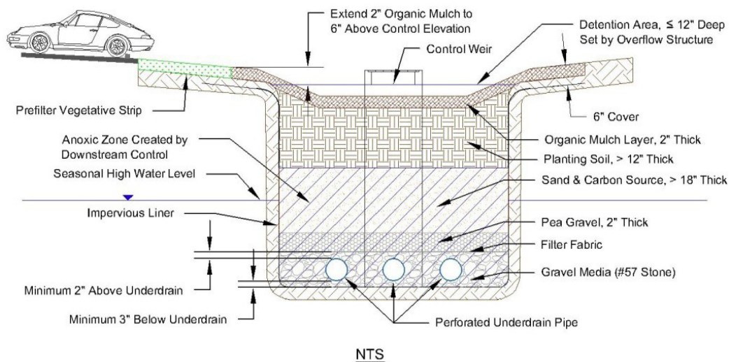
Figure 4.12.2. Cross Section View of a Biofiltration System.
