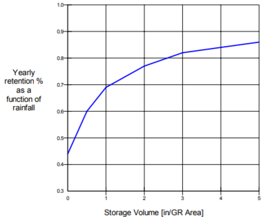
Figure 6.10.1. Green roof Harvesting Design Curve for Tampa Florida Area Using 45 years of data.
