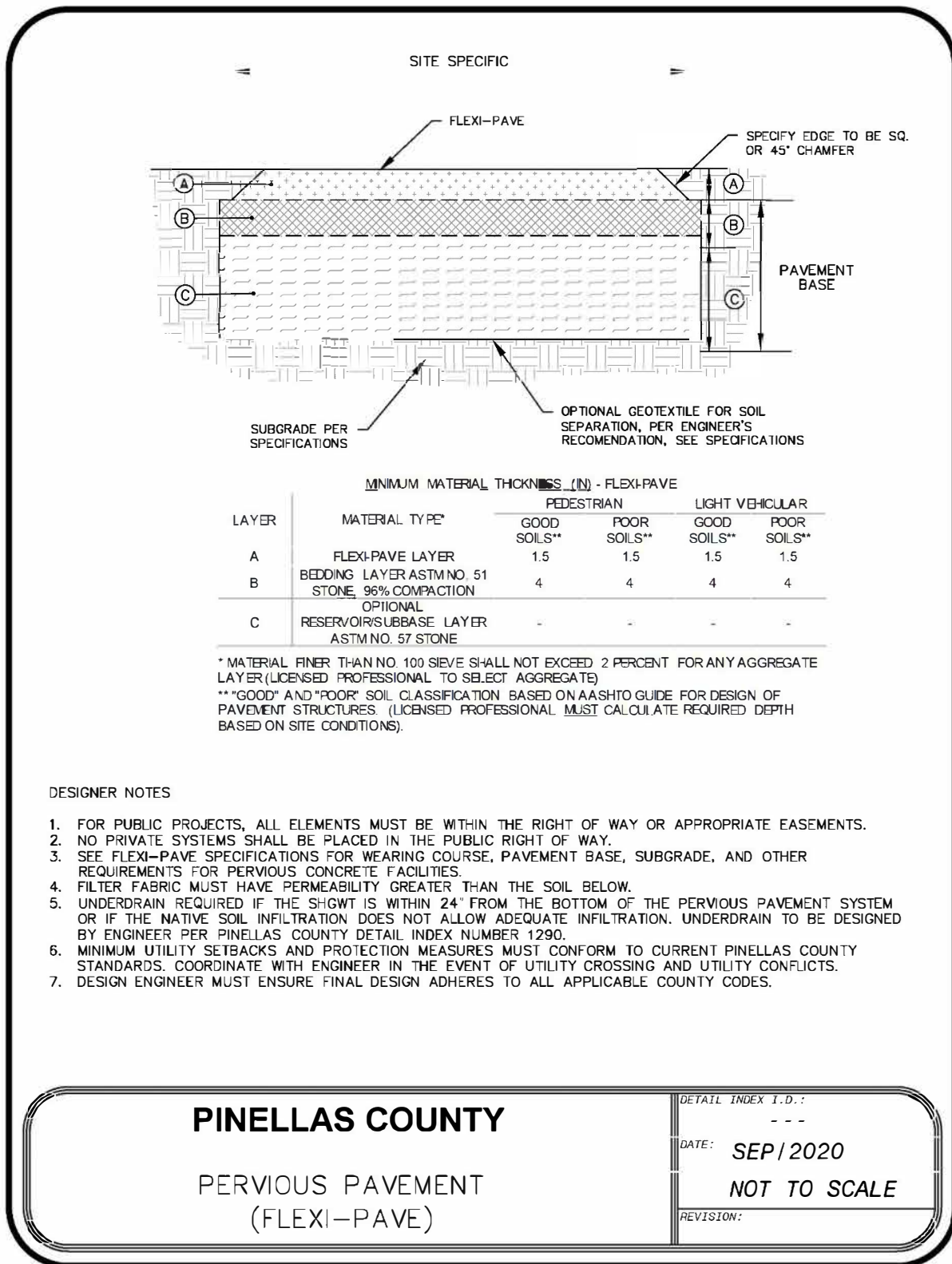
FIGURE 4.6.3.: Pinellas County CAD template for Flexi-Pave™
