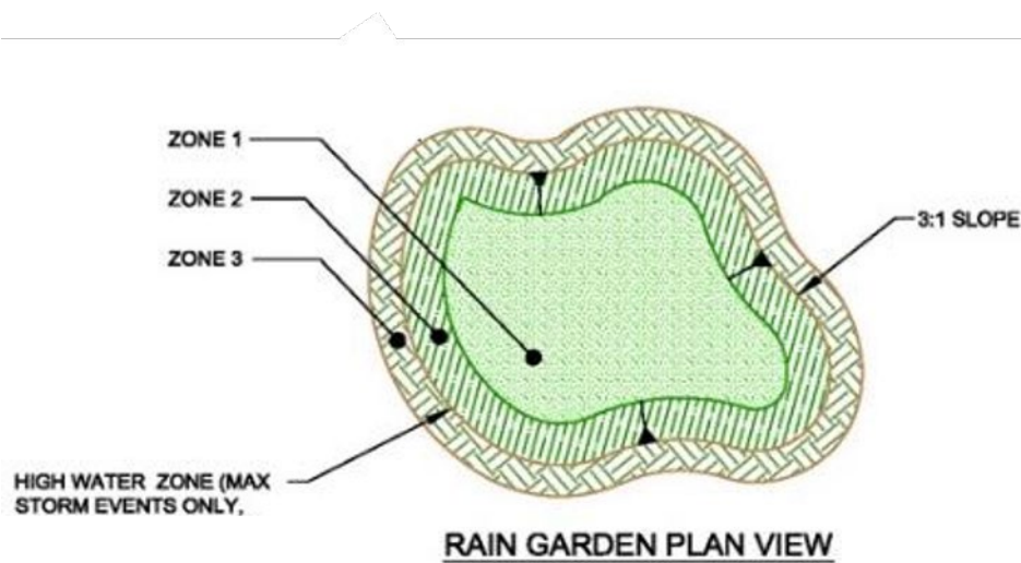
Figure 4.13.3: Rain garden plan view, provided by Applied Sciences, Inc.
