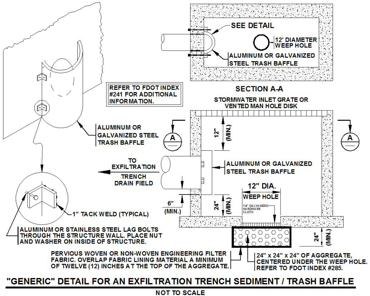
Figure 4.2.4. Detail for Exfiltration Trench Trash Baffle
