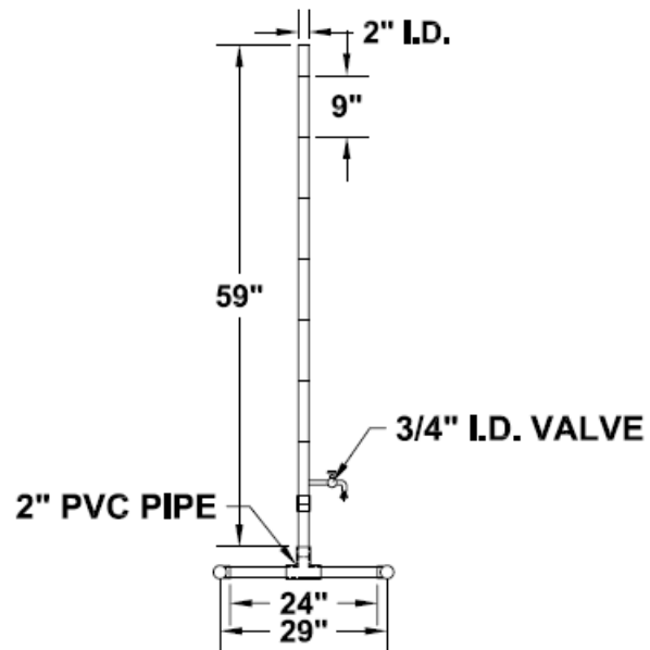
ELEVATION VIEW
